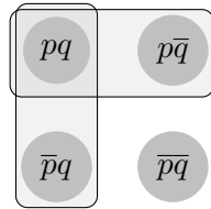
Figure 7.5: p \vee q
