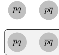
Figure 6.46: [\neg p]^+
