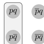
Figure 7.4: p
