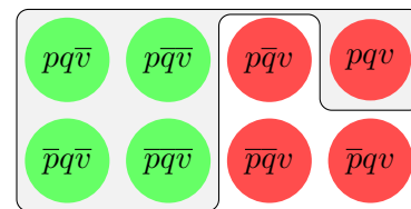
Figure 7.10: \neg\Box(p \wedge q)
