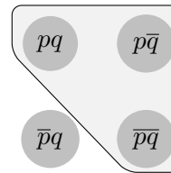
Figure 7.14: q \rightarrow p
