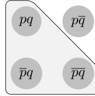
Figure 6.37: [\neg q \rightarrow \neg p]^+
