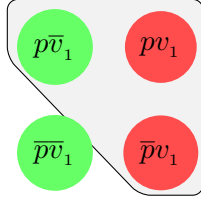
Figure 6.1: \boxed{v_1}p]^+
