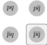
Figure 6.45: [(p \rightarrow q) \wedge \neg q]^+
