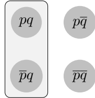
Figure 3.3: q
