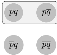
Figure 3.1: p
