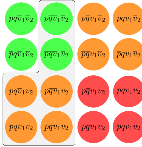
Figure 6.4: [(\diamond_{v_1}(p \vee \neg p)) \wedge (\neg \diamond_{v_2} q)]^+
