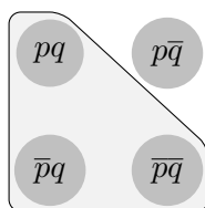
Figure 3.7: p \rightarrow q
