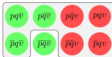
Figure 7.9: \Box(p \vee q)
