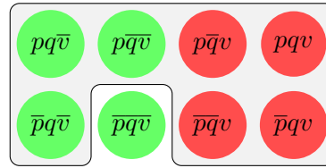
Figure 6.6: [\Box(p \vee q)]^+
