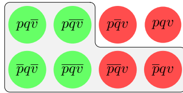
Figure 6.16: [\diamond p]^+
