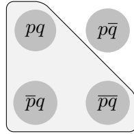
Figure 6.34: p \rightarrow_m q
