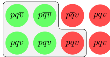
Figure 6.10: [\diamond(p \vee q)]^+
