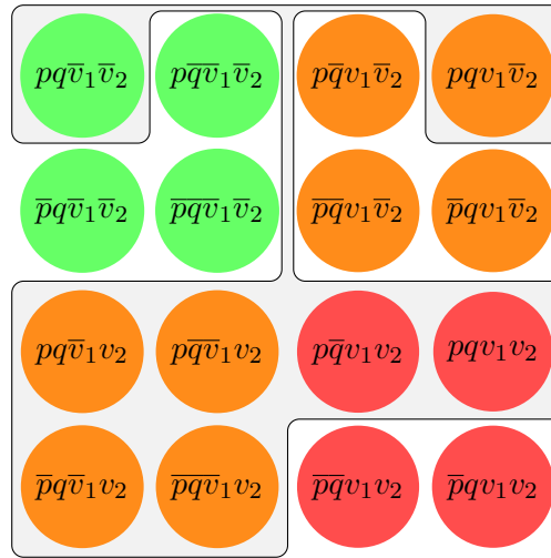
Figure 6.21: [\neg v_1]p \wedge [v_2](p \wedge q)^+
