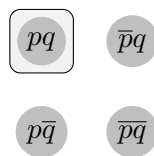
Figure 7.3: p \wedge q
