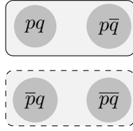
Figure 5.1: p
