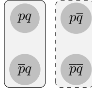
Figure 5.2: q
