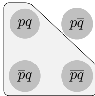
Figure 7.13: p \rightarrow q
