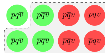
Figure 6.19: [\diamond(p \wedge q)]^-
