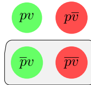
Figure 5.22: [\diamond v p \wedge \neg \diamond v p]^+
