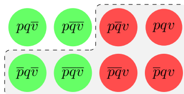
Figure 6.18: [\diamond p]^-
