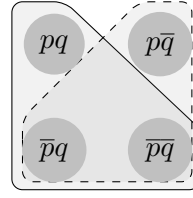
Figure 5.6: p \rightarrow q
