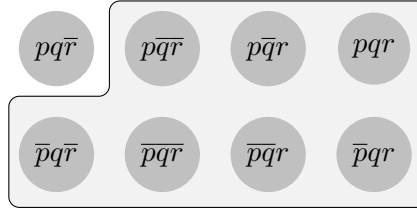
Figure 3.6: (p \wedge q) \rightarrow r
