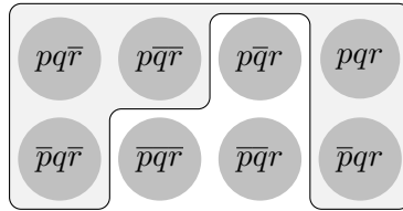
Figure 6.44: [(\neg p \rightarrow (\neg q \rightarrow r)) \wedge (\neg(\neg q \rightarrow r))]^+
