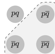
Figure 6.33: [p \rightarrow q]^-
