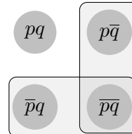
Figure 7.6: \neg(p \wedge q)
