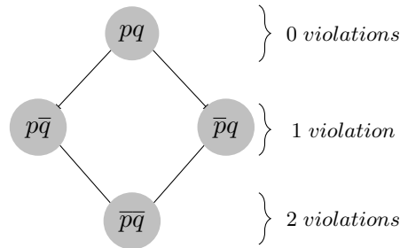
Figure 3.11: \Box p \wedge \Box q
