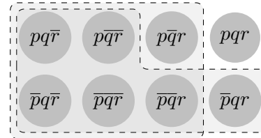
Figure 5.8: [(p \vee q) \rightarrow r]^-
