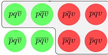
Figure 6.5: [\Box p]^+
