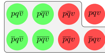
Figure 6.17: [\diamond(p \wedge q)]^+
