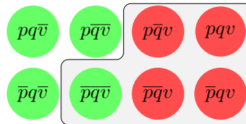
Figure 5.16: [\neg\diamond(p \vee q)]^+
