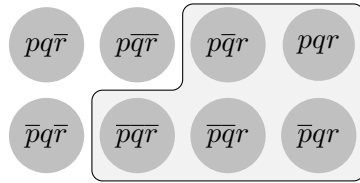
Figure 5.7: [(p \vee q) \rightarrow r]^+
