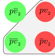
Figure 6.2: \boxed{v_2}\neg p]^+
