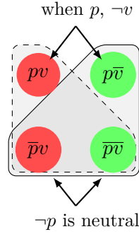
Figure 5.14: \Diamond p/p \rightarrow \neg v
