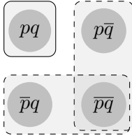
Figure 5.4: p \wedge q
