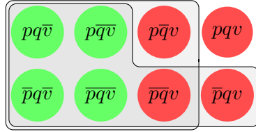
Figure 5.20: [\diamond p \vee \diamond q]^+
