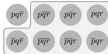
Figure 6.13: [(p \wedge q) \rightarrow r]^+
