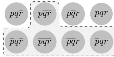
Figure 5.10: [p \rightarrow (q \vee r)]^-
