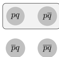
Figure 6.26: p
