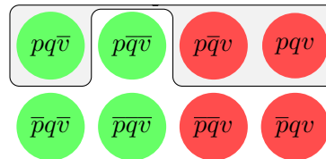
Figure 6.20: [\neg\Box p \wedge \Box(p \wedge q)]^+
