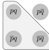
Figure 6.31: p \rightarrow_m q
