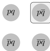
Figure 3.9: \neg(p \rightarrow q)
