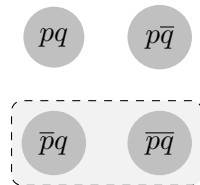
Figure 6.28: [p]^-
