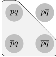
Figure 6.36: [p \rightarrow q]^+
