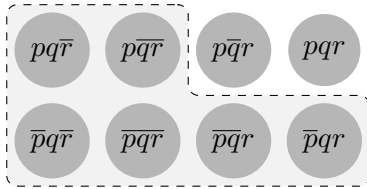
Figure 6.14: [p \rightarrow r]^-
