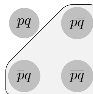
Figure 3.10: p \rightarrow \neg q
