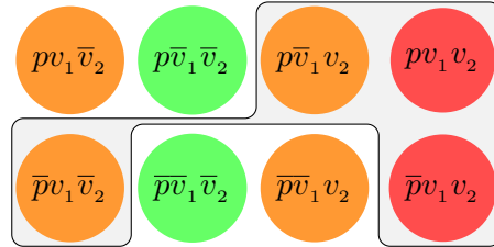
Figure 6.3: \boxed{v_1}p \wedge \boxed{v_2}\neg p]^+
