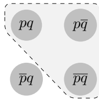
Figure 6.38: [p \rightarrow q]^-
