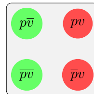
Figure 6.25: [p \rightarrow \Box p]^+
