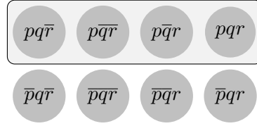
Figure 6.43: p
