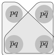
Figure 5.12: p \rightarrow ?q
