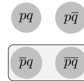
Figure 6.41: \neg p
