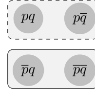
Figure 5.3: \neg p
