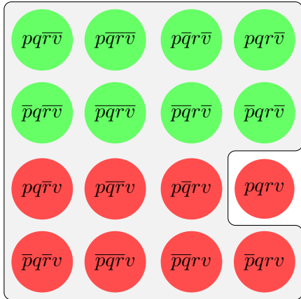
Figure 6.22: [(p \wedge q) \rightarrow \diamond r]^+
