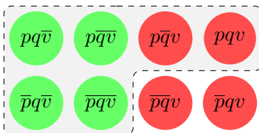
Figure 6.7: [\Box p]^-
