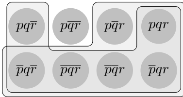
Figure 5.9: [p \rightarrow (q \vee r)]^+
