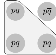
Figure 3.4: p \rightarrow q
