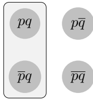
Figure 6.30: q
