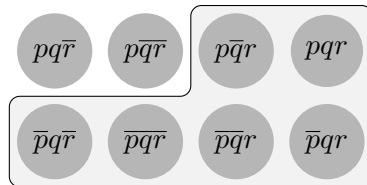
Figure 6.12: [p \rightarrow r]^+
