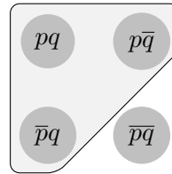
Figure 3.2: \neg p \rightarrow q
