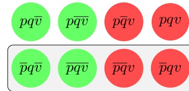
Figure 6.48: [\neg p]^+
