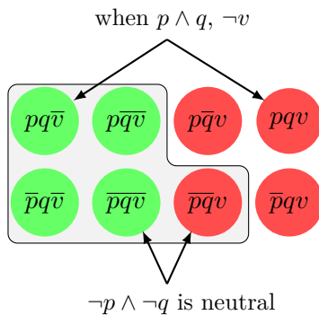
Figure 7.7: \diamond(p \vee q)
