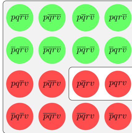
Figure 6.23: [p \rightarrow \diamond r]^+
