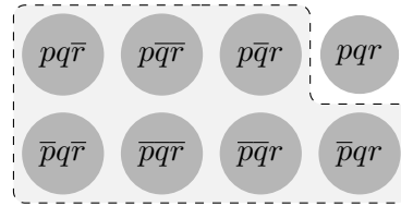
Figure 6.15: [(p \wedge q) \rightarrow r]^-
