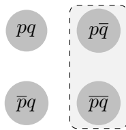
Figure 6.32: [q]^-
