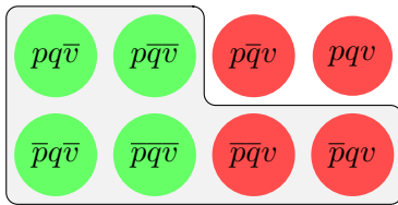
Figure 6.9: [\diamond p]^+
