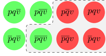
Figure 5.21: [\diamond p \vee \diamond q]^-
