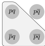
Figure 7.11: p \rightarrow q
