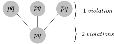
Figure 4.1: \Box p \wedge \Box q \wedge \Box(\neg(p \wedge q))
