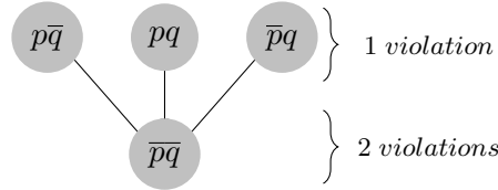
Figure 3.12: \Box p \wedge \Box q \wedge \Box \neg(p \wedge q)
