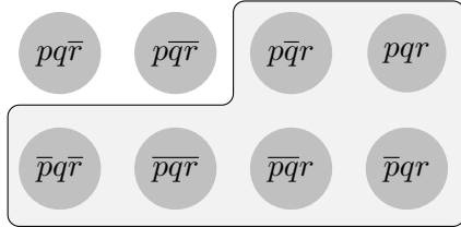
Figure 3.5: p \rightarrow r
