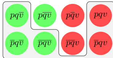
Figure 6.47: [(p \rightarrow (\Box q)) \wedge (\neg \Box q)]^+
